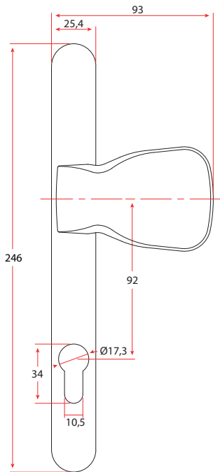
VISTA FRONTAL
